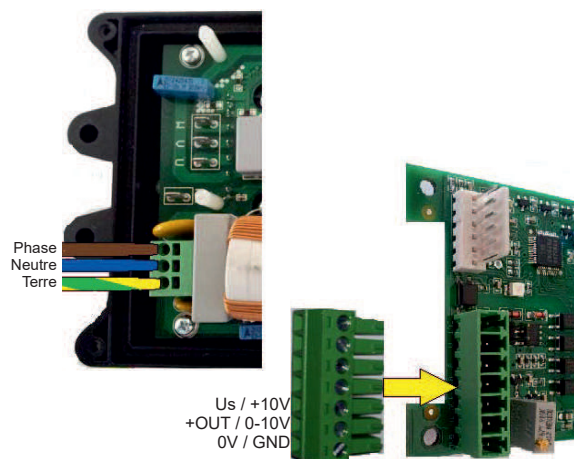
VMI 9/9-4 EC
