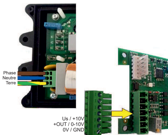
VMI 10/10-4 EC
