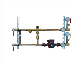
Mixing point and other accessories for coils
