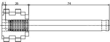
LOA M 150
