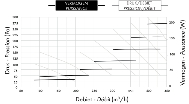
DucoBox Energy D450 m 3 /h
