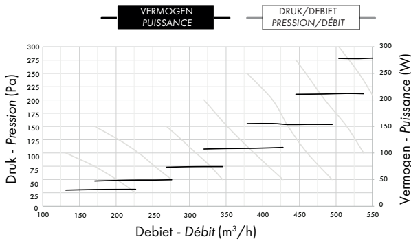
DucoBox Energy D550 m 3 /h
