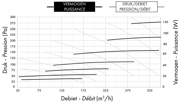
DucoBox Energy D350 m 3 /h
