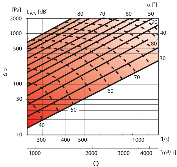
AKH Ø315
