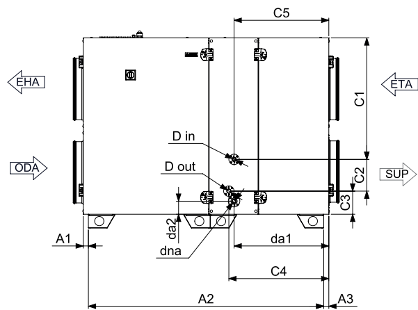
AmberAir Compact S-R H 2000L CO MCB
