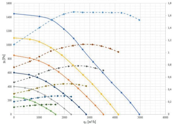
Supply air flow / pressure characteristics
