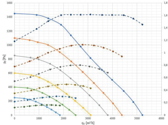
Extract air flow / pressure characteristics
