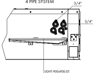
4 PIPE SYSTEM
