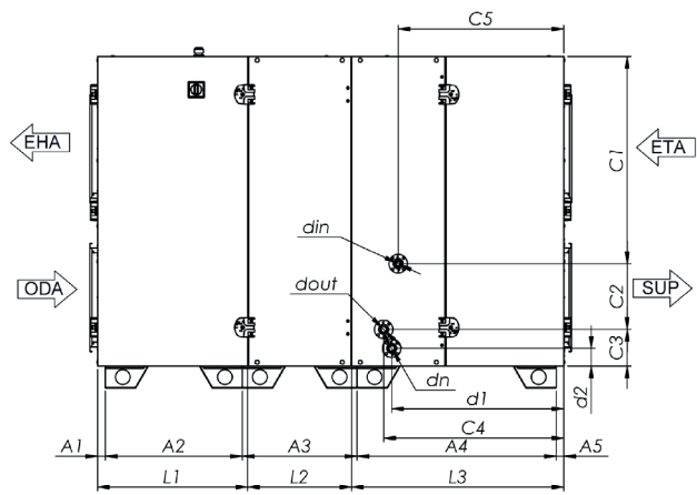
AmberAir Compact S-R H 3000L DX MCB
