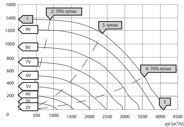
psf [Pa] KCF-N 280 EC 20
