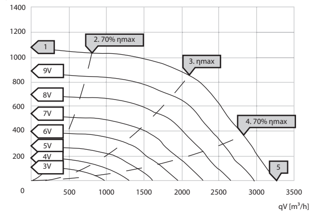
psf [Pa] KCF-N 280 EC 30
