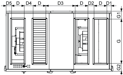
AmberAir Compact S-R V 2000L NB MCB AmberAir Compact S-R V 2000L BE MCB
