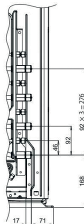
Side view (Valve part)
