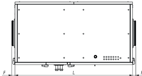
AmberAir Compact S-R H 1000L CO MCB AmberAir Compact S-R H 1500L CO MCB
