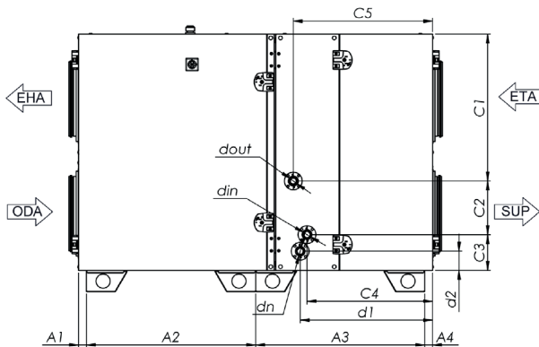
AmberAir Compact S-R H 1000L CO MCB AmberAir Compact S-R H 1500L CO MCB
