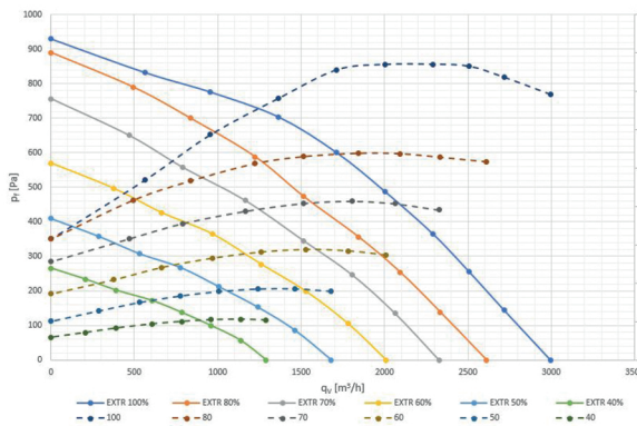
Extract air flow / pressure characteristics
