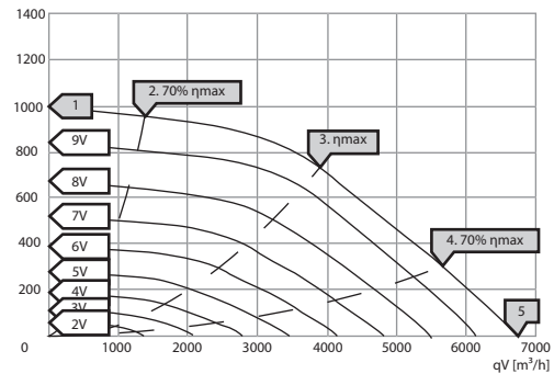
psf [Pa] KBF-N 400 EC T21
