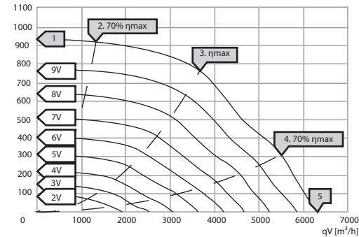
psf [Pa] KBF-N 400 EC T30
