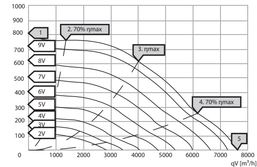
psf [Pa] KBF-N 450 EC T30
