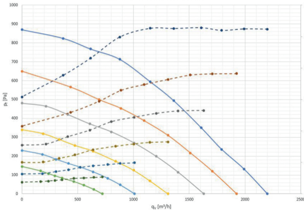
Supply air flow / pressure characteristics
