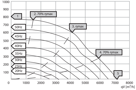
psf [Pa] KBF-N 450 D4 T30
