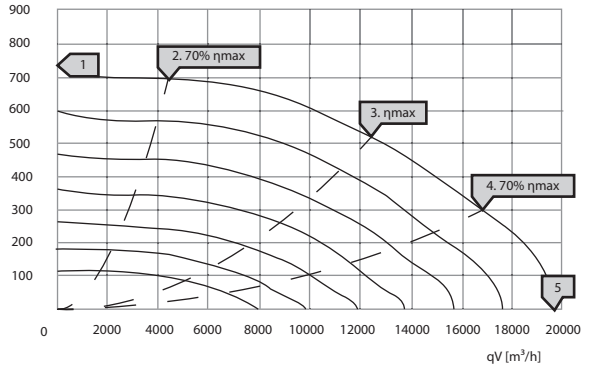
psf [Pa] KBF-N 710 D6 T40
