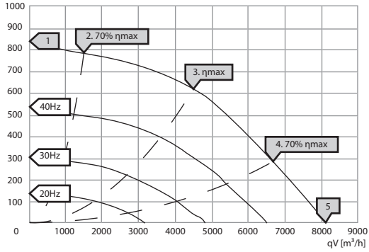
psf [Pa] KBF-N 500 D4 T30
