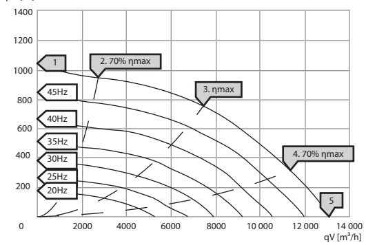
psf [Pa] KBF-N 560 D4 T30
