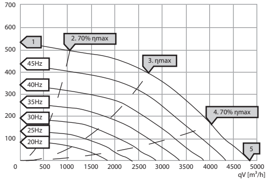
psf [Pa] KBF-N 400 D4 T30
