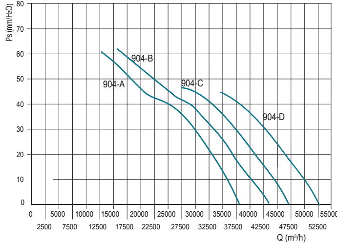
DUCT-M 900 - 4 poles
