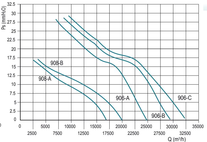
DUCT-M 900 - 6 poles & 8 poles
