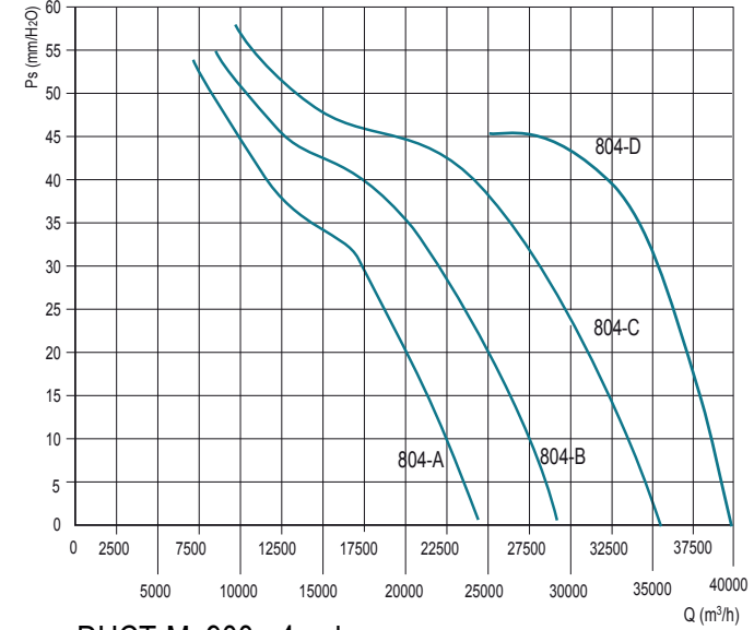
DUCT-M 900 - 4 poles
