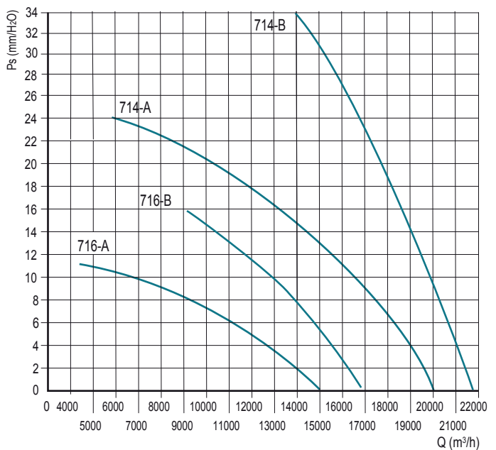
DUCT-M ht 800 - 6 poles
