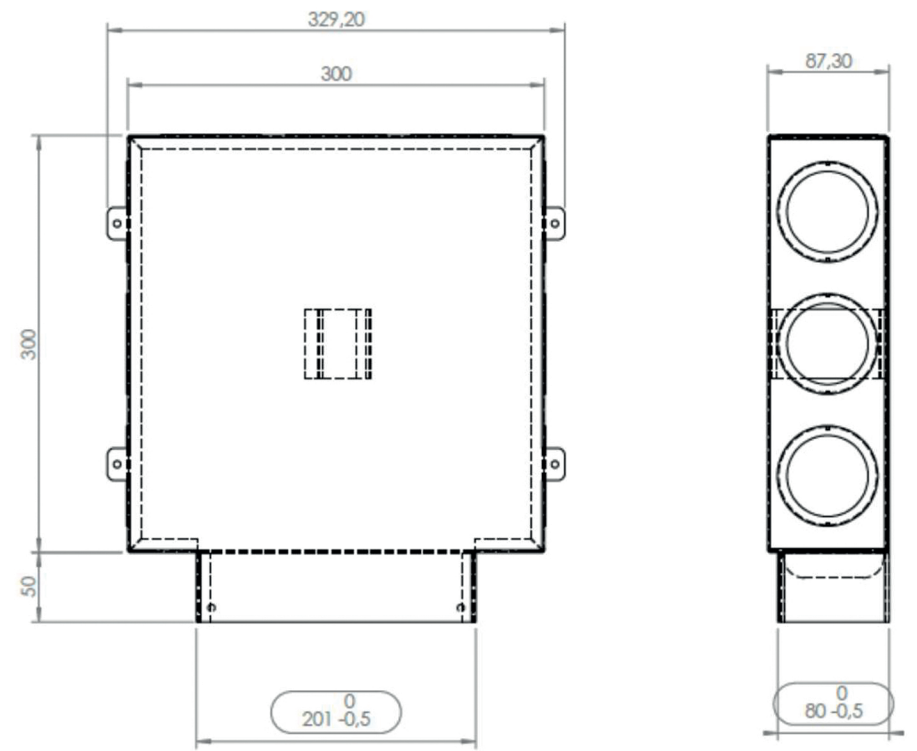
F-COL 180/12x90
