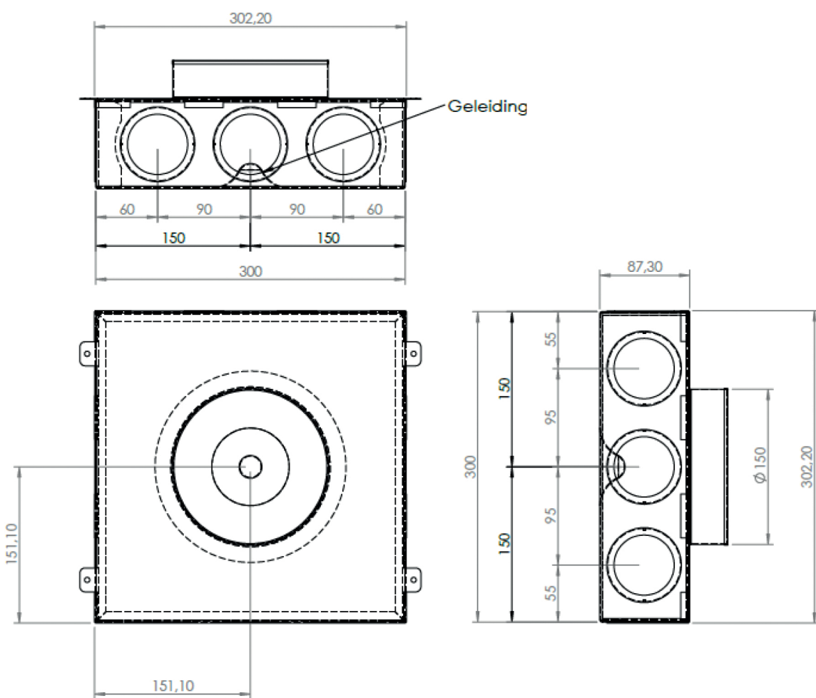
F-COL 150/12x63/70
