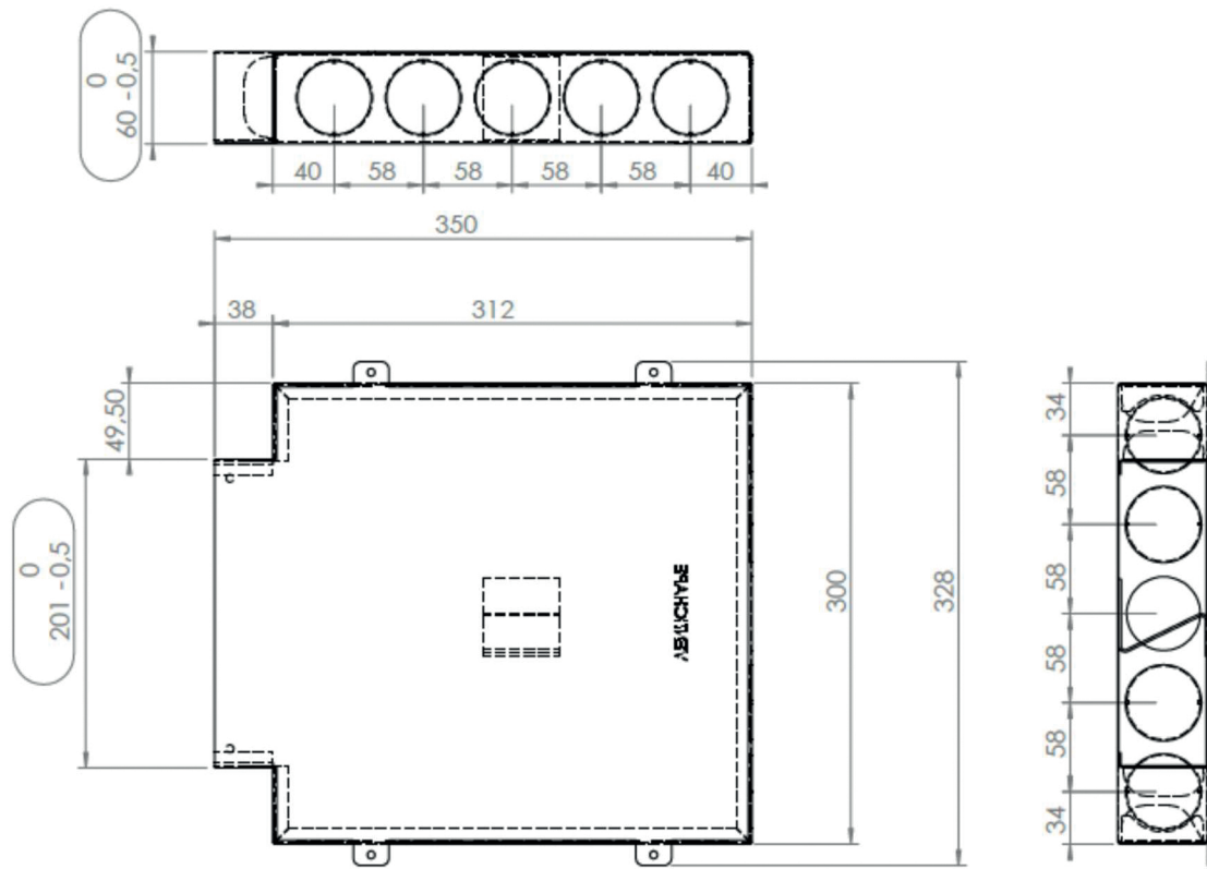
F-COL 150/12x63/70
