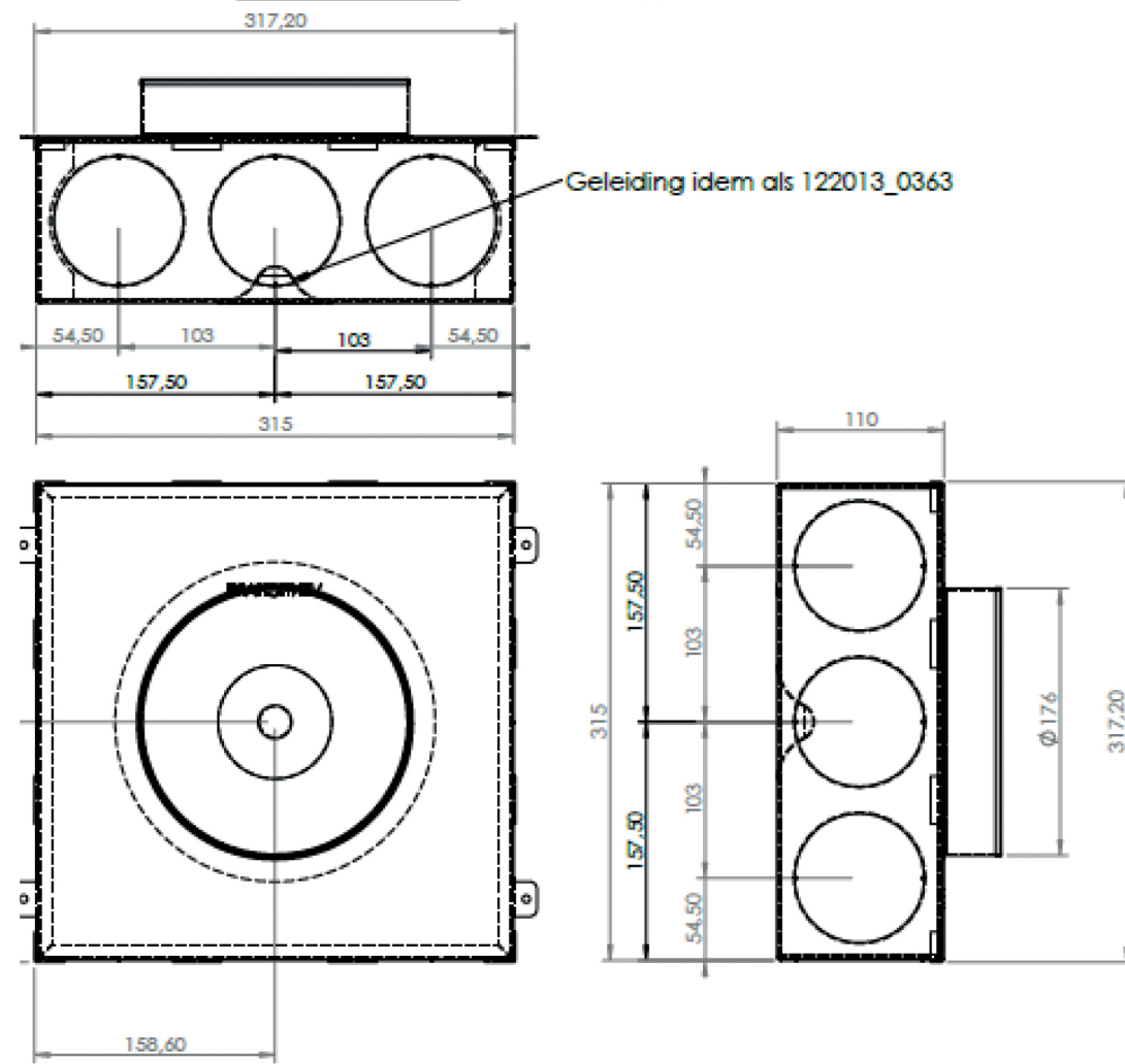
F-COL 180/12x90
