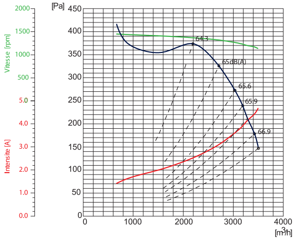
VMI 9/9-4 M
