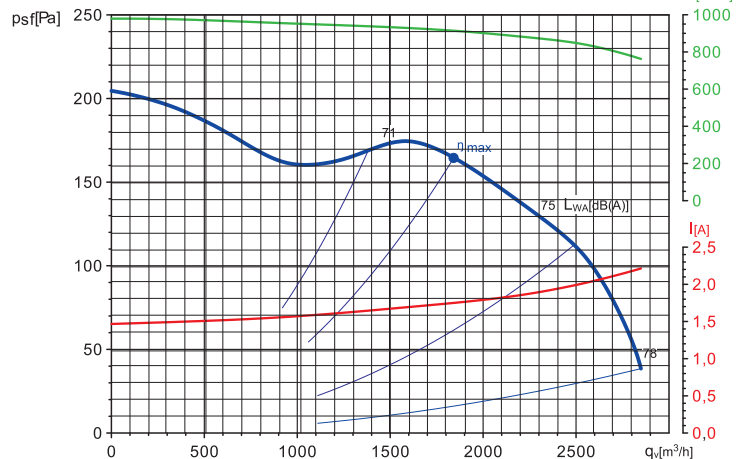
VMI 9/9-6 M
