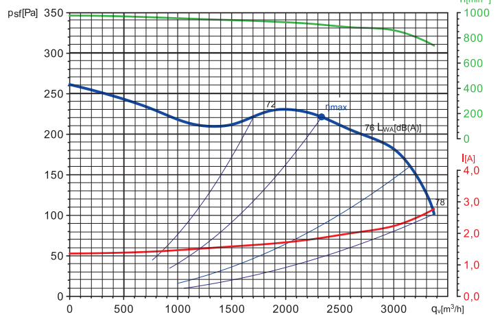
VMI 10/10-6 M
