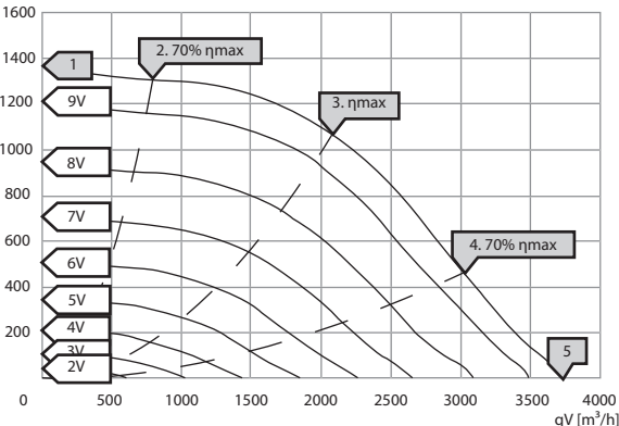
psf [Pa] KBF-N 315 EC T30
