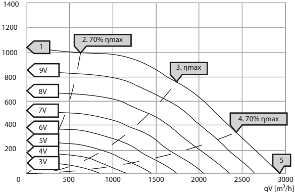
psf [Pa] KBF-N 280 EC T30
