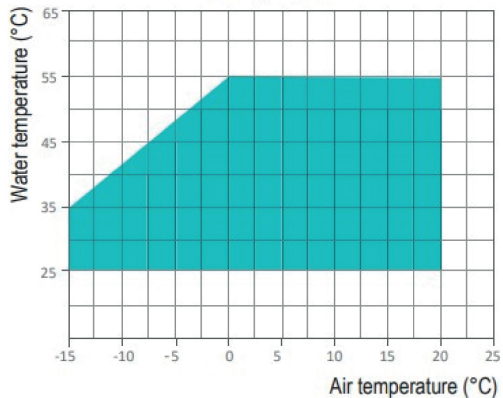
Heating mode
