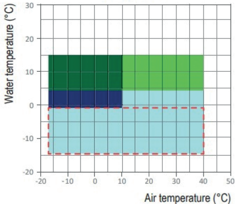
Cooling mode
