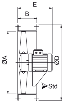
DUCT-Ms ht
