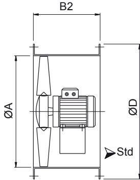
DUCT-MI ht
