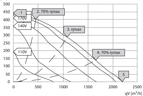
psf [Pa] BFA 355 E2 20
