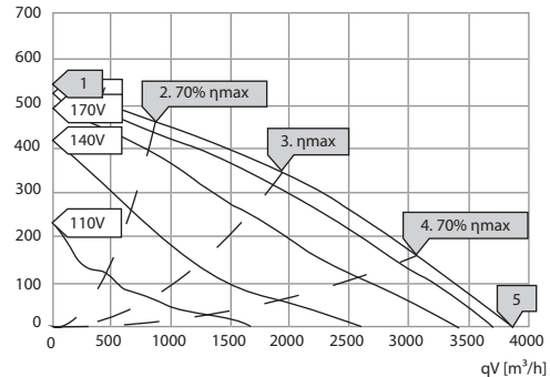
psf [Pa] BFA 500 E2 20
