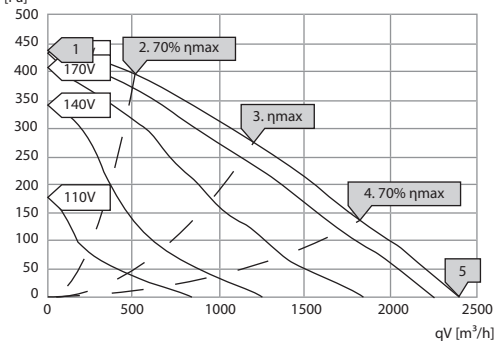
psf [Pa] BFA 400 E2 20
