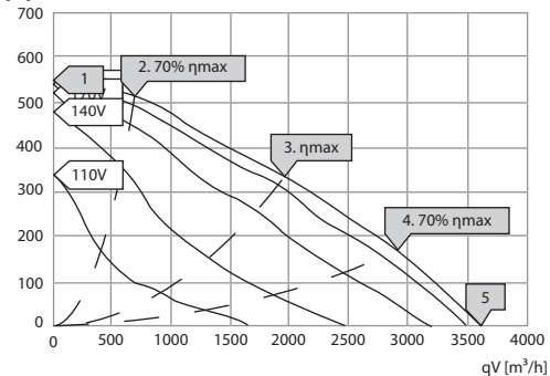
psf [Pa] BFA 450 E2 20
