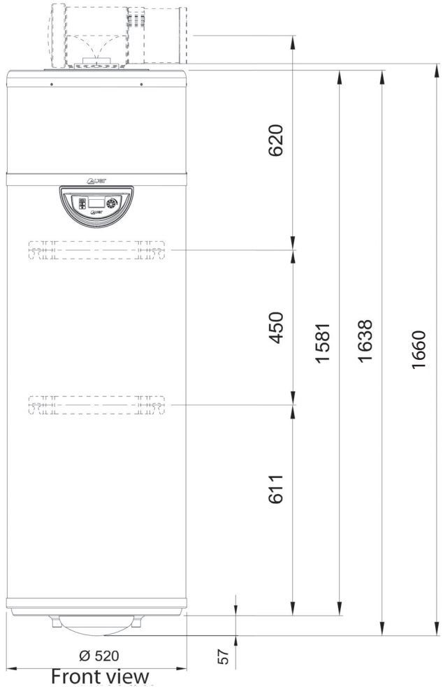
150L Heat pump water heater
