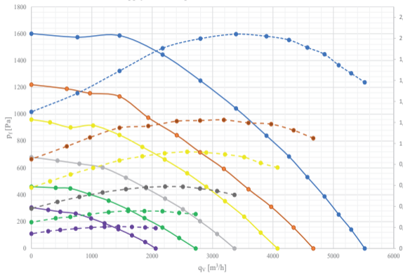
Supply air flow / pressure characteristics
