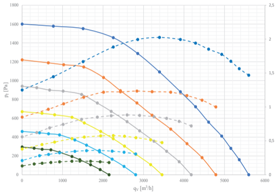
Extract air flow / pressure characteristics
