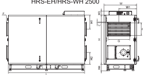
HRS-EH/HRS-WH 2500
