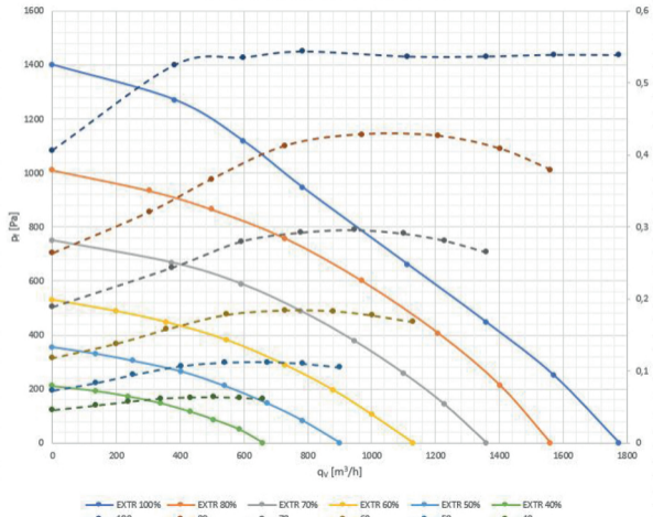
Extract air flow / pressure characteristics
