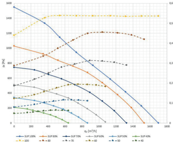
Supply air flow / pressure characteristics
