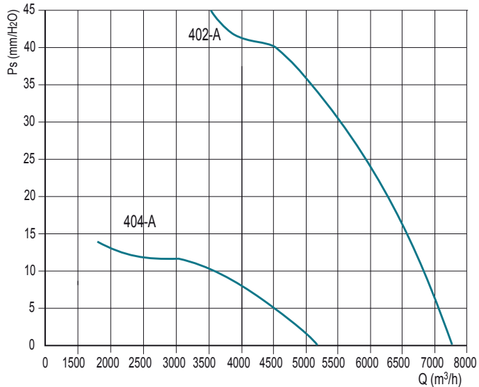
DUCT-M ht 400
