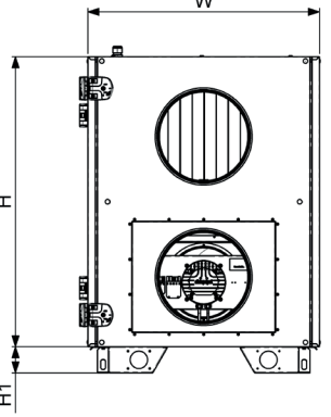
AmberAir Compact S-R H 1000L NB MCB AmberAir Compact S-R H 1000L BE MCB
