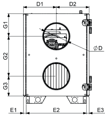
AmberAir Compact S-R H 1500L NB MCB AmberAir Compact S-R H 1500L BE MCB
