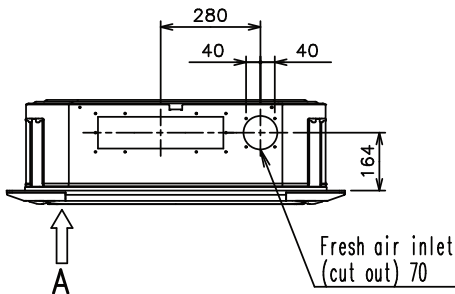
VIEW B
