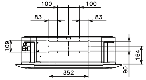
VIEW C
