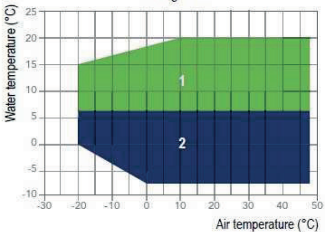
Cooling mode
