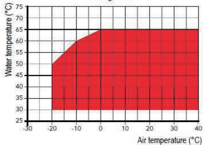
Heating mode
