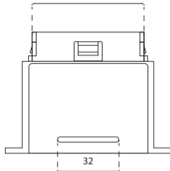
FLEXCON 63
