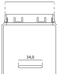
FLEXCON 70
